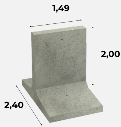
Typ 06 200x149x240 cm 4,125 t
